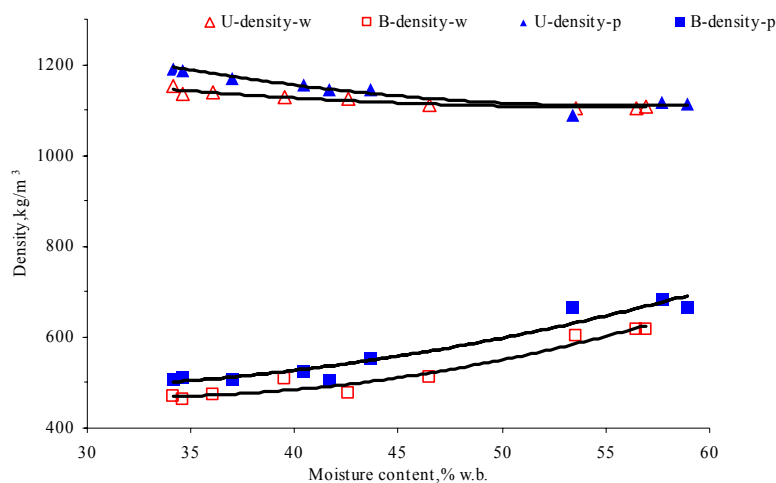
Figure 1. Effect of moisture content on unit and bulk densities of white and pink garlic cloves.
