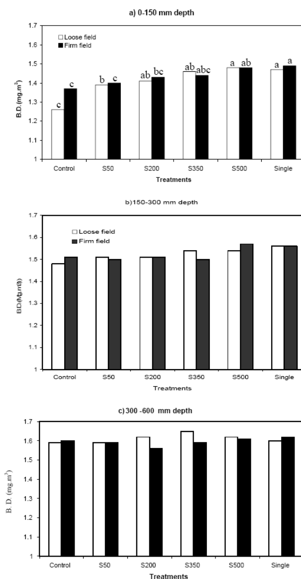
Figure 2. Bulk density ( \text{Mg/m}^3 in both loose and firm fields). S50=50 mm spacing; S200=200 mm spacing; S350=350 mm spacing; S500=500 mm spacing. Similar letter on each column shows no significant difference with 95% confidence.
