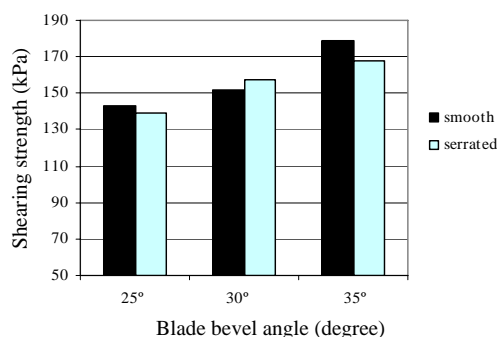
Figure 8. Effect of blade type and bevel angle on the stem shearing strength in the variety Fajr.
