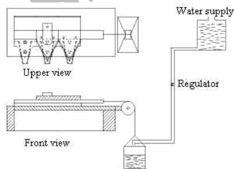
Figure 1. Static shear test apparatus.
