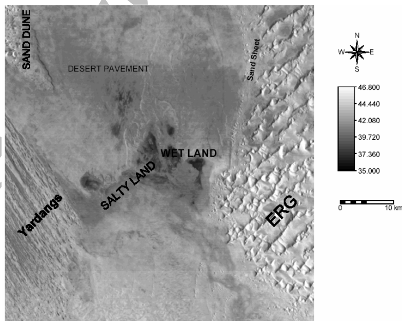
Figure 8. Surface temperature distribution in the Lut Desert derived from the TM band 6 image data the variation of temperature is in Celsius ( ^{\circ} C).
