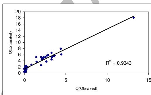
Figure 10. Plot of observed and estimated discharge ( \text{m}^3 \text{s}^{-1} ) for testing.
