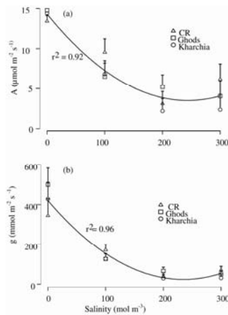
Figure 1. Photosynthesis (A) and stomatal conductance (g) of flag leaves of three wheat cultivars at four levels of salinity. Values represent the mean rate of gas exchange for 8 measurements (two measurements in each replication) made on flag leaf. Vertical lines are confidence intervals of mean values of cultivars.
