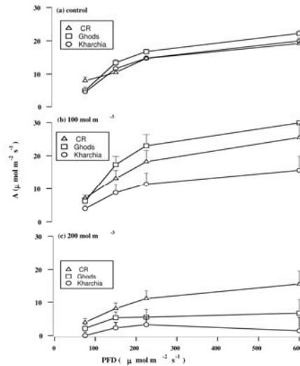
Figure 8. Photosynthesis ( A ) in flag leaves of plants of wheat cultivars grown at control, 100 and 200 \text{mol m}^{-3} salinity and different Photon Flux Densities (PFDs). Each point represents the average of eight measurements (two measurements in each replication). Vertical lines are confidence intervals of mean values of cultivars. Symbols are applicable for all parts of the Figure.
