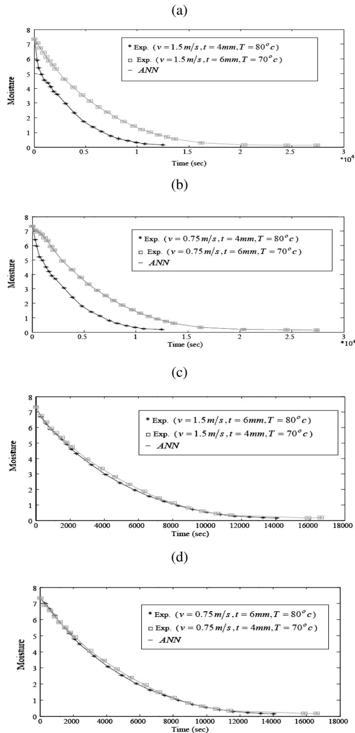
Figure 3. The results of dynamic simulation of moisture during the drying process in terms of temperature, thickness, and air velocity; ANN: 4/4/1 used.
