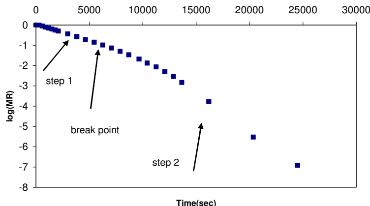
Figure 4. Change of slope in drying curve.
