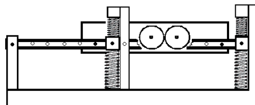
Figure 1. Vibration simulator.
