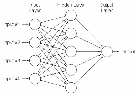
Figure 4. An artificial neural network with one hidden layer.
