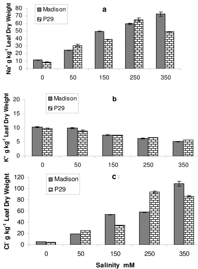
Figure 4. Leaf sodium ( \text{Na}^+ ), potassium ( \text{K}^+ ) and chloride ( \text{Cl}^- ) concentrations ( \text{g kg}^{-1} dry weight) after 8 weeks exposure to different salt concentrations. Each bar is the average of six replications. Vertical lines are standard error of the means.
