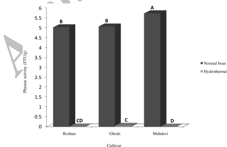
Figure 3. Comparison of phytase activity of normal and hydrothermaled brans obtained from three Iranian wheat cultivars.
