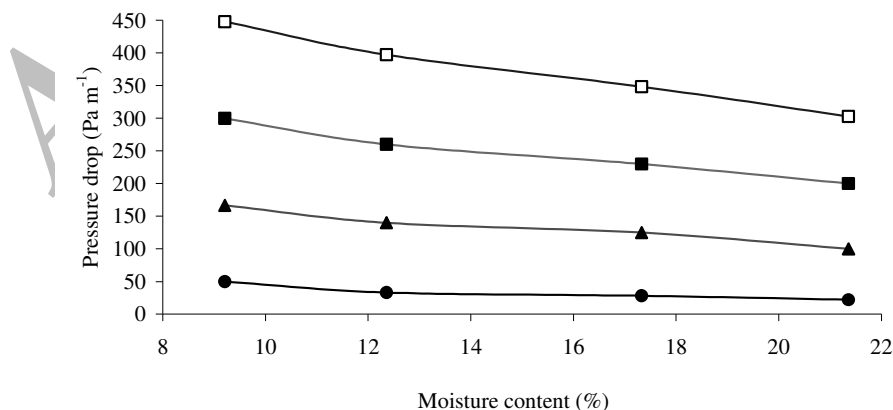
Figure 4. Pressure drop vs. moisture content for chickpea seeds in loose fill test column at airflow rates of: 0.1 (●), 0.2 (▲), 0.3 (■) and 0.4 (□) \text{m}^3 \text{s}^{-1} \text{m}^{-2} .
