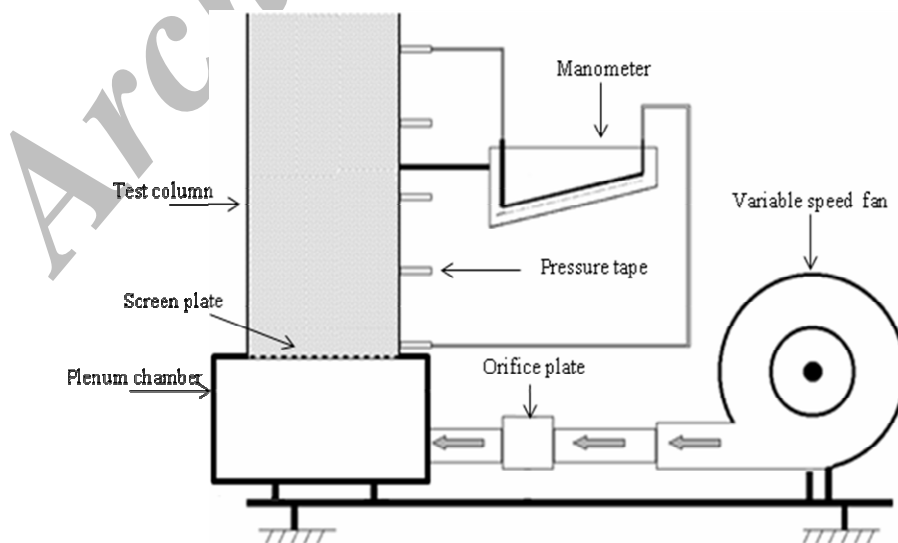
Figure 1. Schematic diagram of the apparatus used for measurement of the airflow resistance of chickpea seeds.
