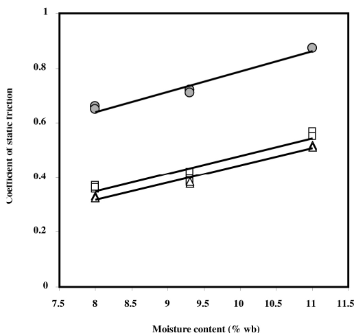
Figure 3. Effect of moisture content on coefficient of static friction of alfalfa ground with hammer mill screen size of 4.76 mm: ● = Rubber surface; □ = Galvanized iron surface; △ = Plexiglass surface.
