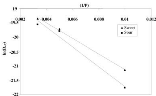
Figure 13. Variation of \ln(D_{eff}) with (1/P) for sweet and sour pomegranate arils in microwave drying.
