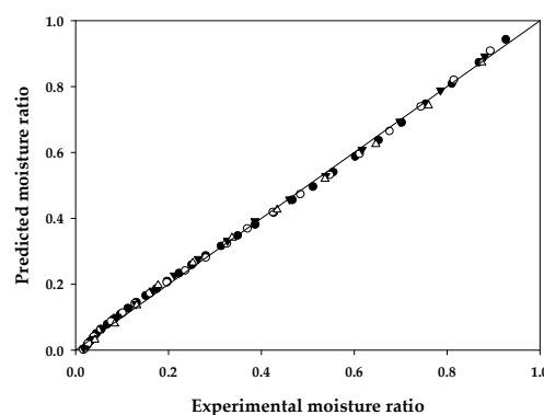
Figure 4. Comparison of experimental and predicted moisture ratio by the logarithmic model: ● (T= 50°C), ○ (T= 60°C), ▼ (T= 70°C), △ (T= 80°C)
