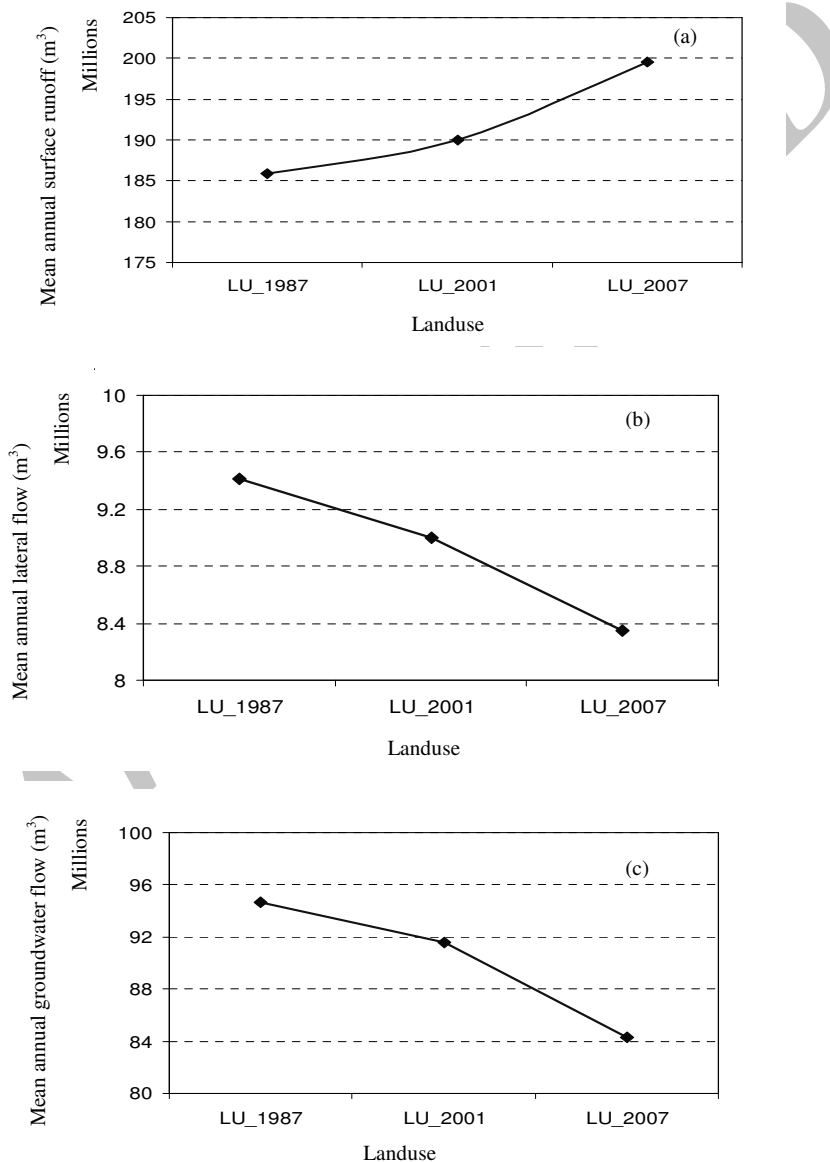
Figure 5. Effects of land use changes in the years 1987, 2001, and 2007 on the mean annual (a) surface runoff, (b) lateral flow and (c) groundwater flow.
