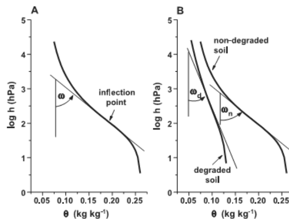
Figure 1. Example of a soil moisture retention curve and its slope at the inflection point (from Dexter, 2004).
