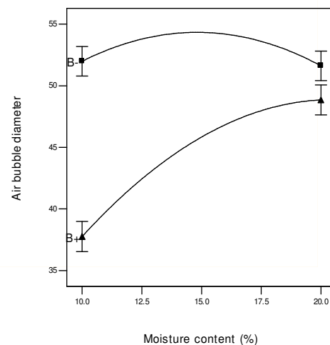
Figure 4. Effect of moisture content and corn grain genotype on air bubble diameter ( \mu\text{m} ) of the popcorns obtained by experimental modeling from the Design Expert. (SquaresB-: American grain, Triangles B+: Hybrid grain)
