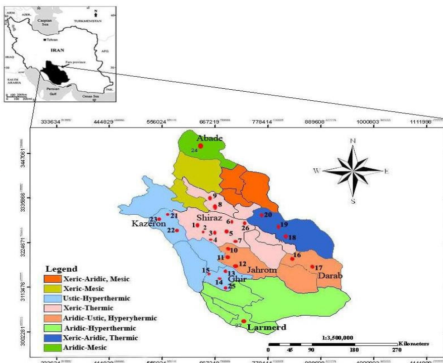
Figure 1. Soil moisture regimes and location of soil pedons in the study area.
