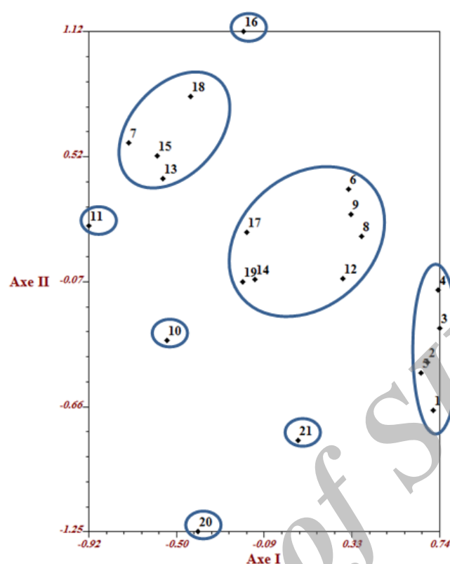
Figure 3. Nonmetric multidimensional scaling analysis of Jaccard coefficient between 21 accessions of pomegranate (The Stress value is 0.071).
