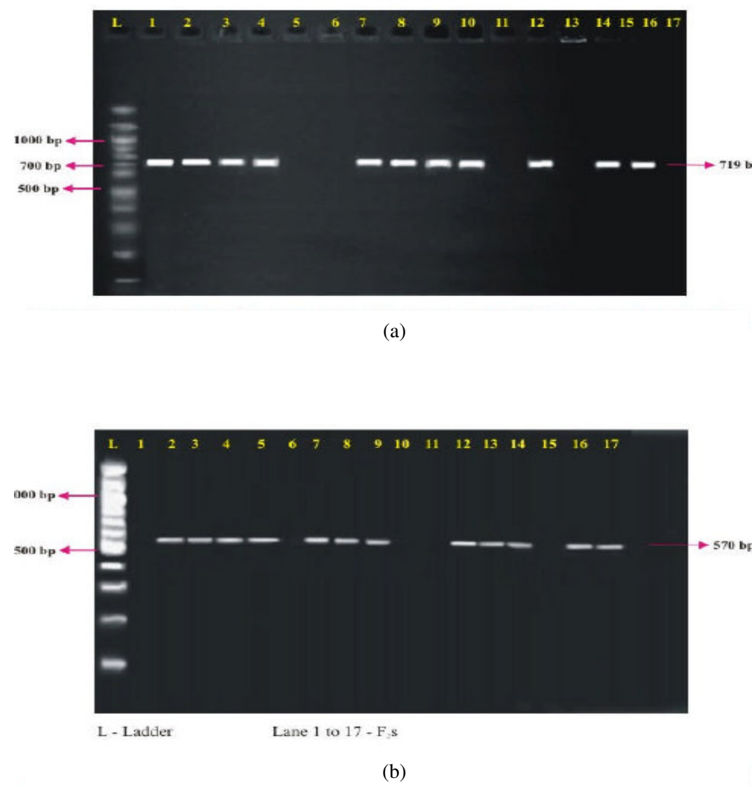
Figure 1. Genotyping of F 2 population of the cross MP-3299×NIL PBW-343 using SCAR marker SCS73719 linked to Lr24 gene. (a) Lane no. 16 is NIL PBW-343 and Lane no. 17 is MP 3299. (b) Lane no. 1 is MP 3299 and Lane no. 2 is NIL PBW-343.
