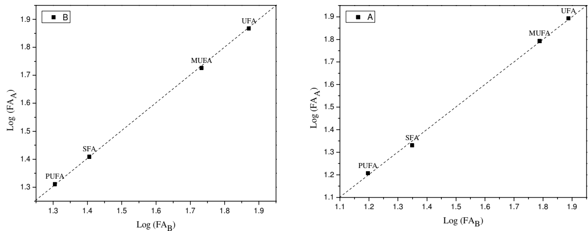
Figure 3. Relationship between the content of total Unsaturated Fatty Acids (UFAs), Saturated Fatty Acids (SFAs), MonoUnsaturated Fatty Acid (MUFA), PolyUnsaturated Fatty Acid (PUFA) before and after the refining process. (FA B = % of fatty acid before the refining process; FA A = % of fatty acid after the refining process; B: Bladi sample, A: Arbequina sample).
