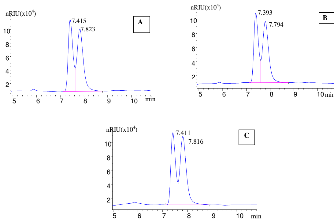
Figure 2. HPLC chromatograms of sugars: (A) Date syrup; (B) Date concentrate, and (C) Date liquid sugar. The peaks at about 7.4 and 7.8 min are for glucose and fructose, respectively.
