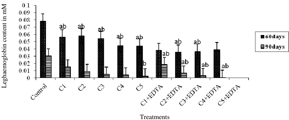
Figure 4. Effect of different concentration of Chromium with and without EDTA on leghaemoglobin content (mM) on Sesbania grandiflora . Significant difference at P \leq 0.01 (a); P \leq 0.05 (b), significant difference at P \leq 0.01 , and P \leq 0.05 (ab).
