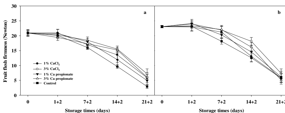
Figure 3. Fruit firmness in (a) ‘Bagheri’, and (b) ‘Asgarabadi’ apricot cultivars after treatment with 1 and 3% CaCl 2 or Calcium propionate at harvest and storage at 1°C. Means±Standard error (n= 4).
