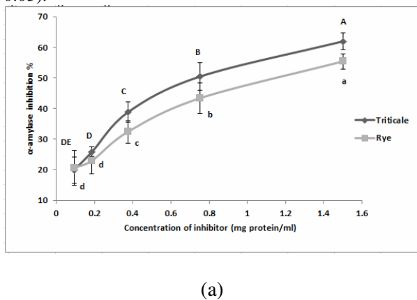
Figure 4. Inhibition of potato tuberworm \alpha -amylase (a) and protease (b) by different concentrations of triticale and rye. Means followed by the same letters are not significantly different by Tukey's test ( P < 0.05 ).
