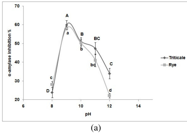
Figure 3. The effect of pH on inhibition of potato tuberworm \alpha -amylase (a) and protease (b) by extracts from triticale and rye. Means followed by the same letters are not significantly different by Tukey's test ( P < 0.05 ).
