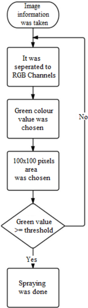
Figure 6. Flow diagram of spraying weeds between rows.
