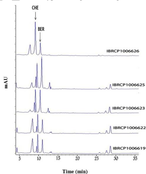
Figure 4. Separated chelidonine and berberine chromatograms from leaves of five Iranian C. majus ecotypes at vegetative stage.
