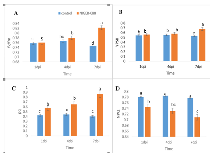
Figure 3. Chlorophyll fluorescence parameters in citrus leaves treated with Xcc : (A) Potential quantum efficiency of PSII (Fv/Fm); (B) PSII operating efficiency (YPSII); (C) Photochemical fluorescence quenching (qp); (D) Nonphotochemical Fluorescence Quenching (NPQ) of control and Xcc -infiltrated citrus leaves at the times stated. The results are the mean of three replicates and error bars represent the standard deviations.
