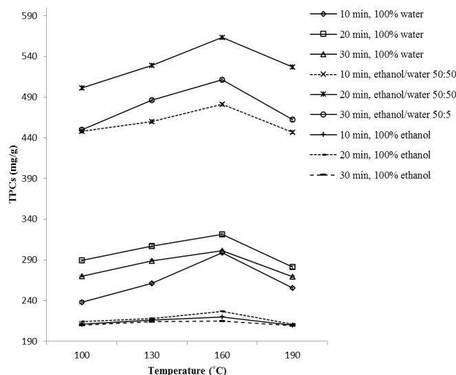
Figure 3. The effect of extraction temperature, time and ethanol/water ratio of SSE method on extraction yield of PPEs
