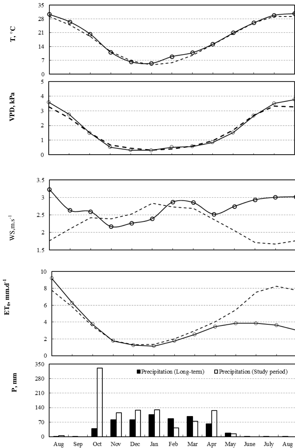
Figure 4. Monthly mean climate data for the study period (August 2015-August 2016), solid marked line, versus long-term (1986–2016), dashed line, as recorded by the nearby Meteorological Station in Ilam. From the top to bottom, Temperature (T), Vapor Pressure Deficit (VPD), Wind Speed (WS), reference Evapotranspiration (ET 0 ), and Precipitation (P).
