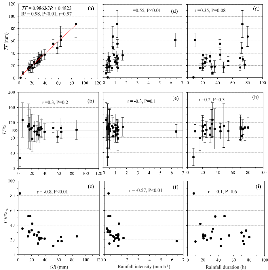
Figure 4. The correlation between mean values of throughfall ( TF ), TF% , CV% OTF with (a, b, c) gross rainfall ( GR ) amount, (d, e, f) rainfall intensity, (g, h, i) and rainfall duration for individual rainfall events. Bars indicate \pm standard error.
