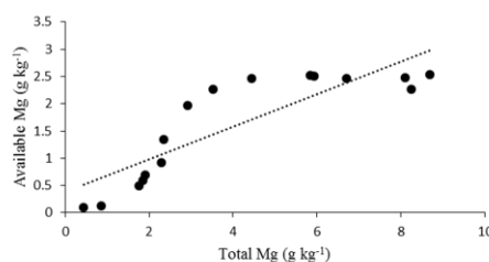
Figure 6. Relationships between available and total concentration of Mg of TwBC, WhBC, WsBC and ApBC at four pyrolysis temperatures.
