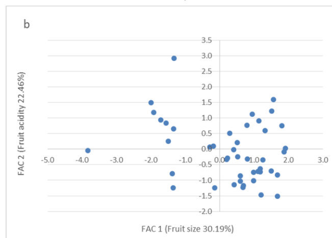
Figure 4. The Principal Component Analysis (PCA): (A) The first three-factor for the variables and (B) Scatter biplot of (FAC1 and FAC2) for the non-affected and affected genotypes of AB disorder in pomegranate genotypes.
