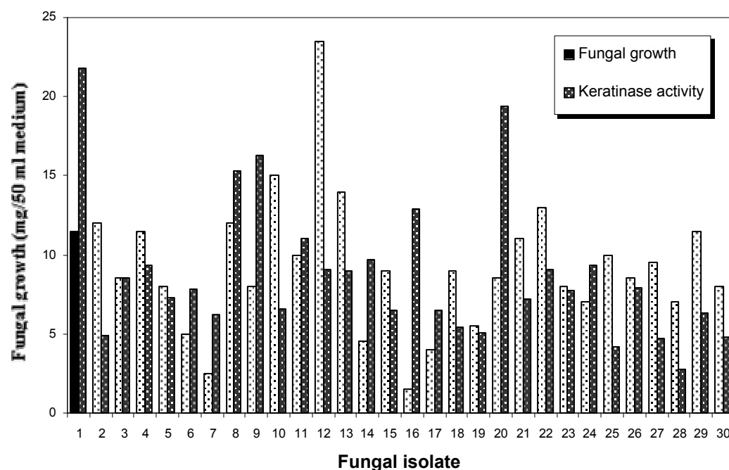
Fig. 2. Comparison of growth rate and extracellular keratinase activity in Trichophyton mentagrophytes isolates maintained in
