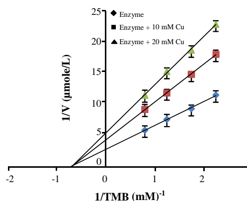
Fig. 2. Lineweaver-Burk reciprocal plot of the myeloperoxidase activity versus the reciprocal concentration of tetramethyl benzidine in the absence ( \blacklozenge ), or 10 mM ( \blacksquare ) and 20 mM ( \blacktriangle ) concentrations of copper, as an inhibitor. Each point represents the average of three measurements. behavior of MPO in vitro .
