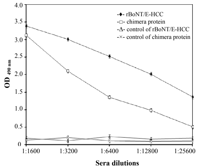
Fig. 3. ELISA results of rabbit serum antibody titration against rBoNT/E-HCC and chimer proteins. Both anti-rBoNT/E-HCC and anti-chimer protein sera from rabbits bind to their antigens up to 1:25,600; however, anti-rBoNT/E-HCC (recombinant C-terminal heavy chain of BoNT/E) serum had higher affinity. Serum from non-immunized rabbit did not react with either rBoNT/E-HCC or chimer protein. The error bars present high reproducibility of double repeats of the experiment.
