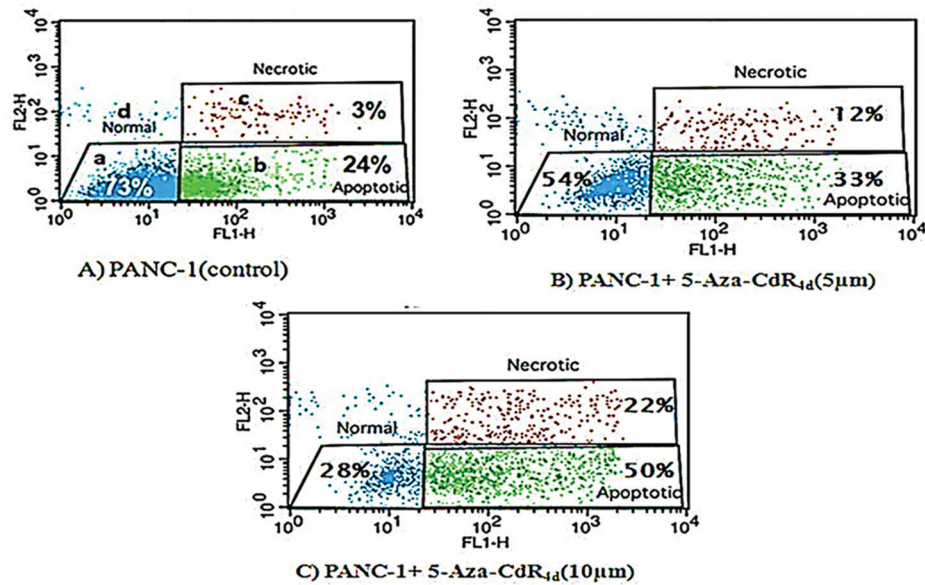
Figure 3: (A) Untreated PANC-1 (control), (B) PANC-1 treated with 5 \mu M of 5-AzaCdR, (C) PANC-1 treated with 10 \mu M of 5-Aza-CdR. The (a) quadrant indicates viable cells, which are negative for annexin-V and PI staining. The (b) quadrant shows apoptotic cells that take up annexin-V and stain green, while negative for PI staining. The (c) quadrant represents late apoptotic cells that are annexin-V and PI positive. The (d) quadrant represents necrotic cells, which are annexin-V negative and PI positive staining.
