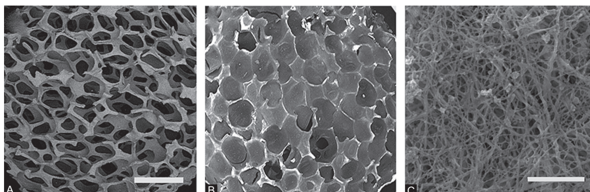
Figure 2: Scanning electron micrographs at low magnification show good porosity in the HA/ZrO 2 scaffold (A). Pores are also filled with PRP/HS (B). PRP scaffold contains randomly oriented fibrin fibers and platelets. It also contains nano-sized pores (C). Scale bar is 2.5 mm for A and B and 5 µm for C.
