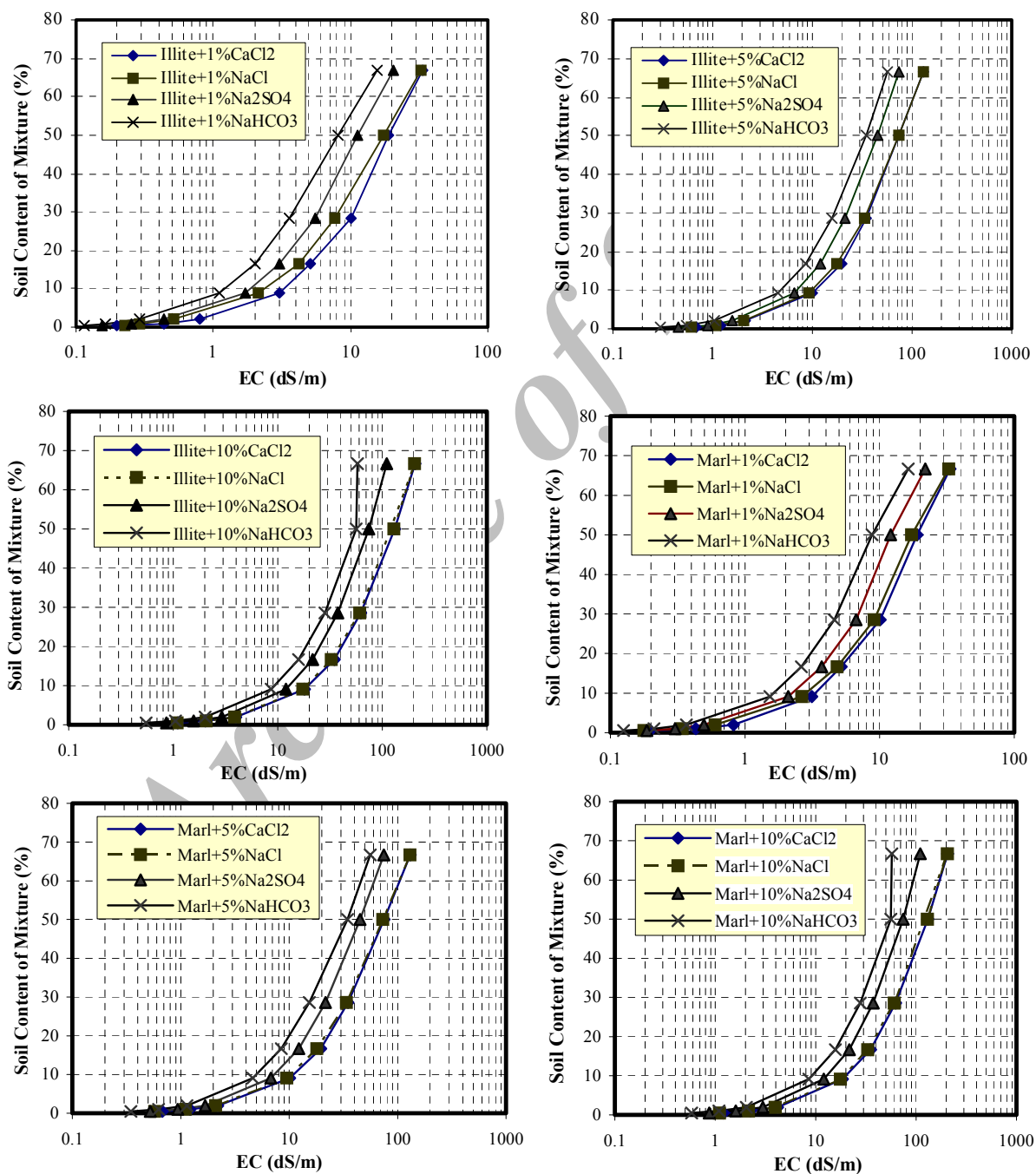
Fig. 5. Anion type effect on EC of marly soil and illite
