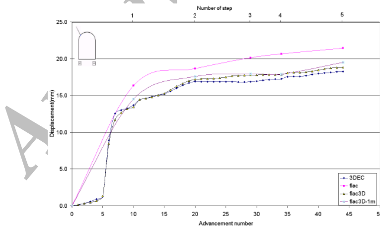
Fig. 7. Deformations in the U/S of roof in powerhouse for different steps
