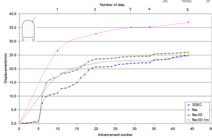
Fig. 6. Deformations in the center of roof in powerhouse for different steps
