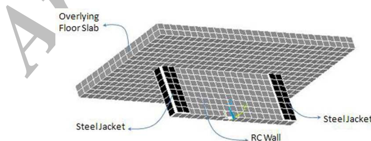
Fig. 5. Finite element model of RC wall strengthened by steel jackets
