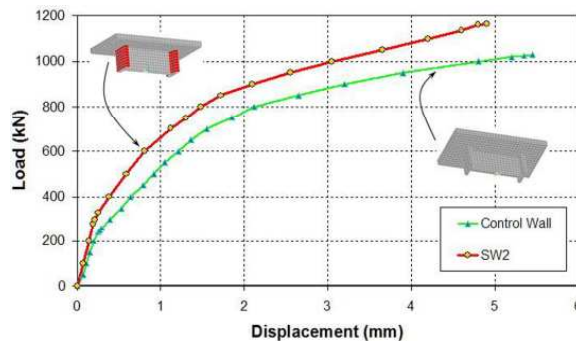
Fig. 10. Comparison of FE analysis load-displacement curves for the “Control wall” and “Strengthened wall with two vertical CFRP layers”
