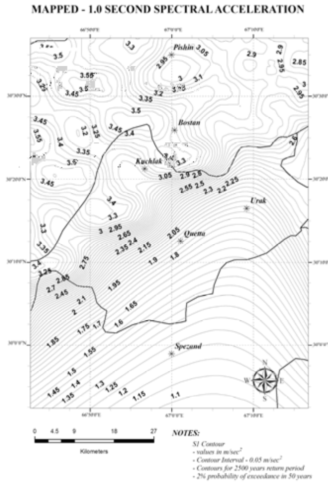
Fig. 3. 1-second spectral acceleration contours for 2500 years return period
