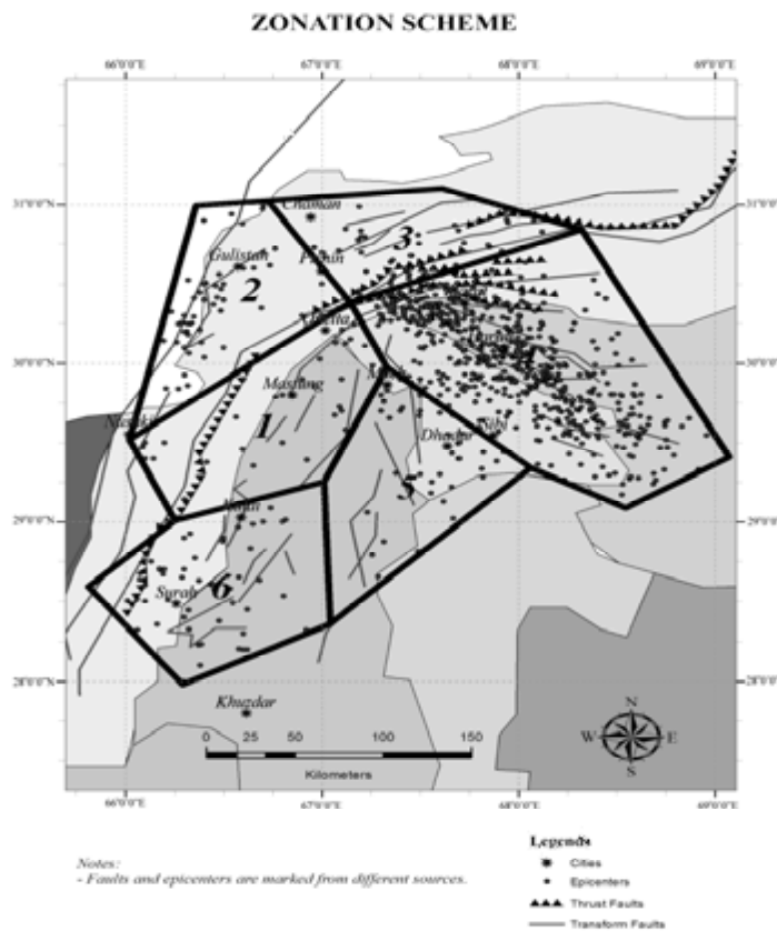
Fig. 1. Micro-zonation scheme for the area; marking of epicenters and faults in each seismic source zone
