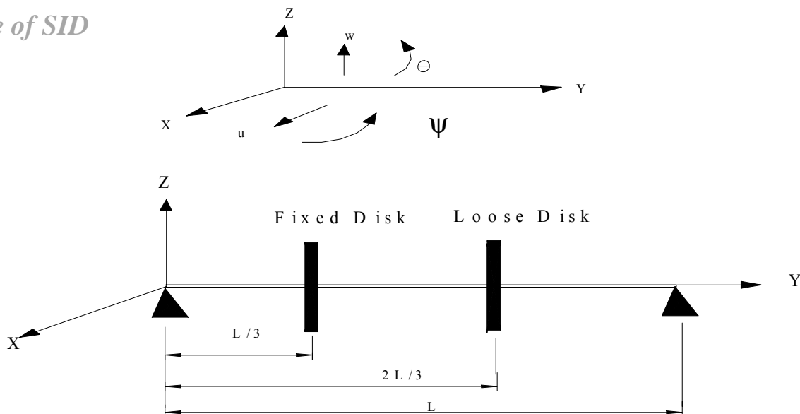
Figure 3. Rotor-Bearing system with loose disk.
