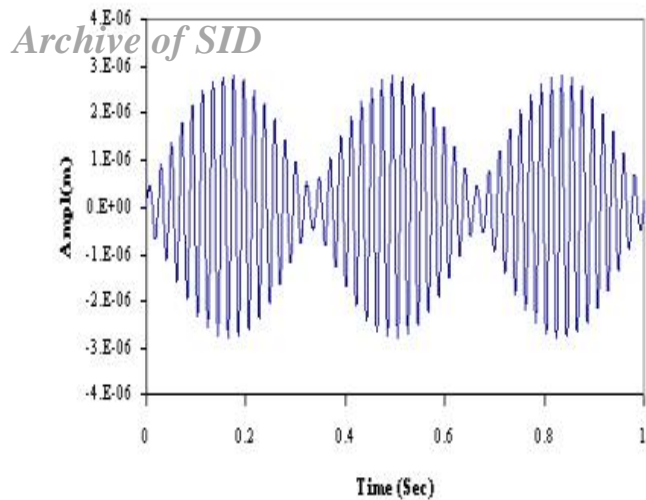
Figure 5. The system response due to unbalance effect for analytical solution.
