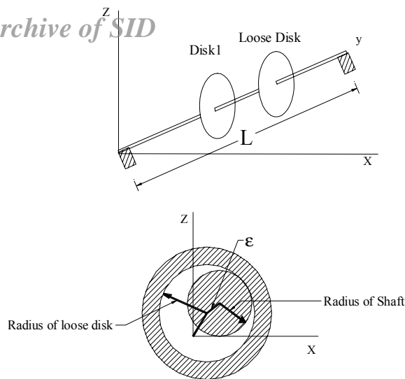
Figure 1. Rotor with loose disk.
