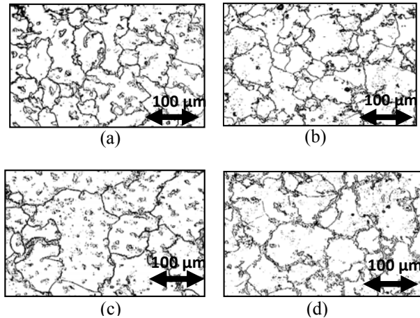
Figure 3 Microstructures of the as-cast F-75 alloys with the mold preheating at: (a) 550 °C, (b) 700 °C, (c) 850 °C and (d) 1000 °C.
