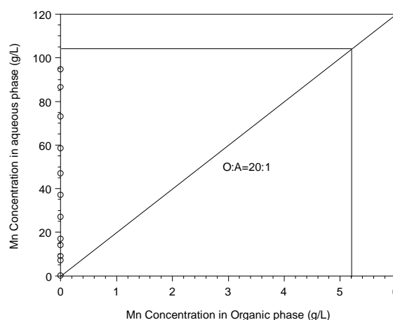
Figure 8. McCabe-Thiele plot for stripping of manganese loaded D2EHPA using 180 g/L H 2 SO 4 .
