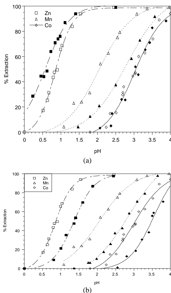
Figure 1. Effect of pH on extraction of zinc, manganese and cobalt. Hollow symbols are related to 0.6 M D2EHPA. Solid symbols correspond to 0.3 to 0.3 mixture of D2EHPA and Cyanex ® having a fixed extractant concentration of 0.6 M, for: (a) Cyanex ® 302 (b) Cyanex ® 272
