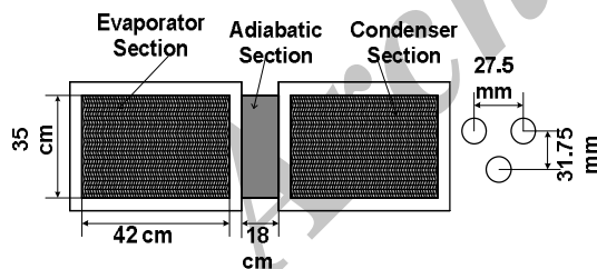
Figure 1. (a) Schematic diagram of the test set-up, and (b) Schematic of the HPHX and tube arrangements
