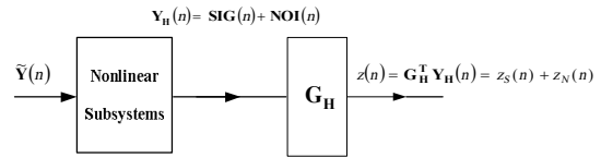
Figure 3. Hammerstein combiner
