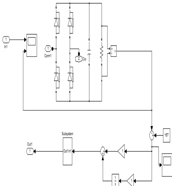
Figure 8. Subsystem 1 of Closed Loop Control of Voltage Sag Compensation in a DVR System
