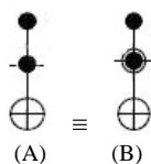
Figure 5. Use of the Peres gate instead of the Toffoli gate. (A) TG, (B) PG
