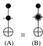
Figure 5. Use of the Peres gate instead of the Toffoli gate. (A) TG, (B) PG
