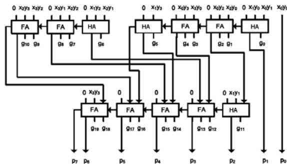
Figure 2. 4x4 reversible multiplier circuit in which output of PPGC are input of parallel adder
